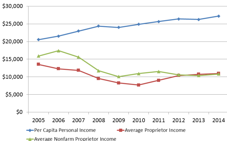
Per Capita Personal Income versus Average Proprietor Income Prentiss County
